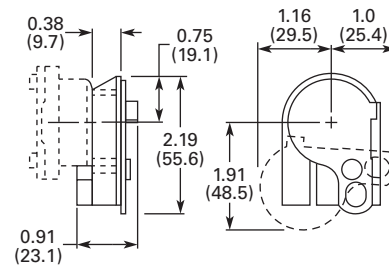
Padlock Attachment for Maintained Push-Pull Operator Catalog No. 10250TA64
