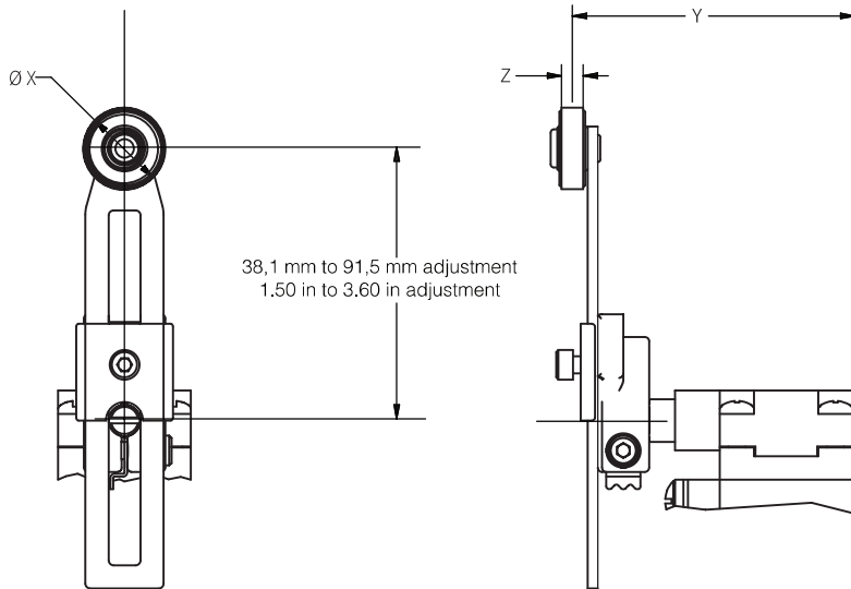
Figure 5. Aluminum Rod Lever Dimensions, GLZ54
