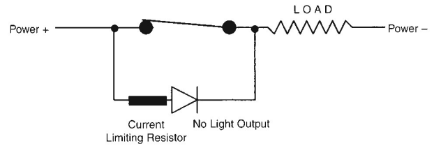
Figure 17. Wiring Diagram 2
