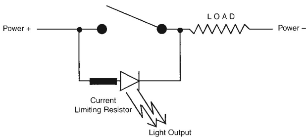
Figure 16. Wiring Diagram 1
