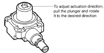
Figure 14. Actuation Adjustment
