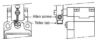
Figure 13. Allen Screw and Teller Tab Location
