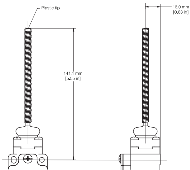
Figure 9. Coil Actuator
