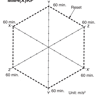
MM4(X)KP
