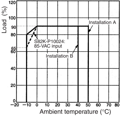
100-W Models with PFC (S82K-P10024) Parallel-Unit Operation
