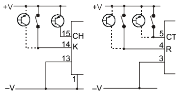
Ingressi Source (PNP)
