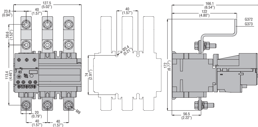
RF...420 thermal relay with links
