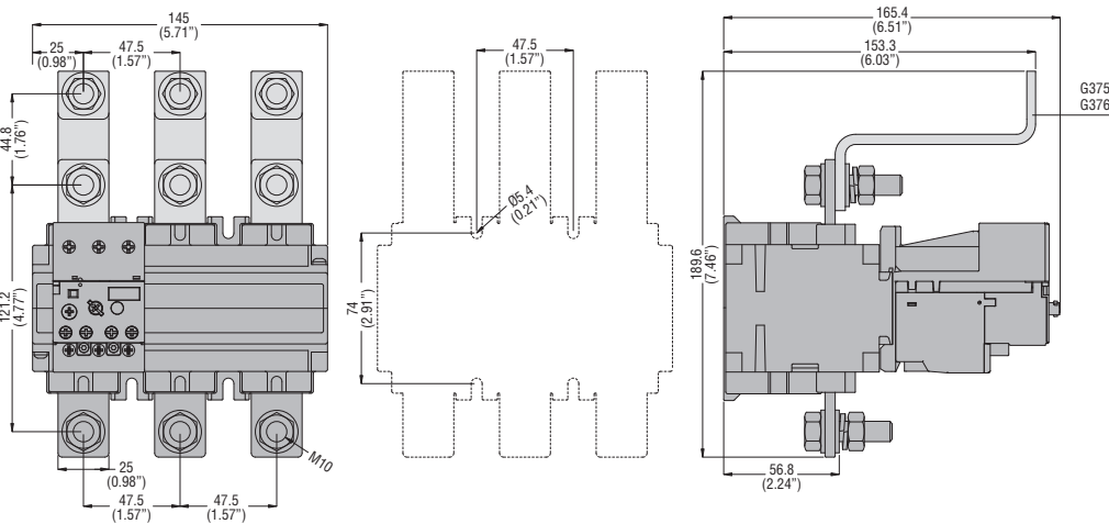
RF...420 thermal relay with links
