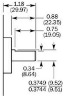
3/8" w/Flat
