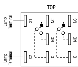
Screw Terminal
