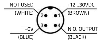
M12 PIGTAIL
