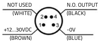
RECEIVER F
