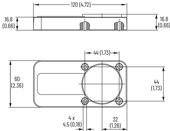
Figure 5 - Actuator [mm (in.)]
