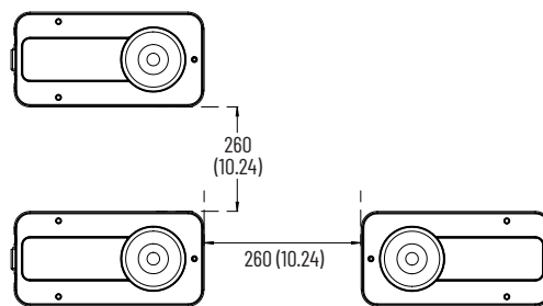
Figure 1 - Spacing Requirement [mm (in.)]
