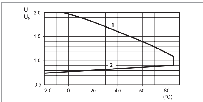
R 55 - DC coil operating range v ambient temperature
