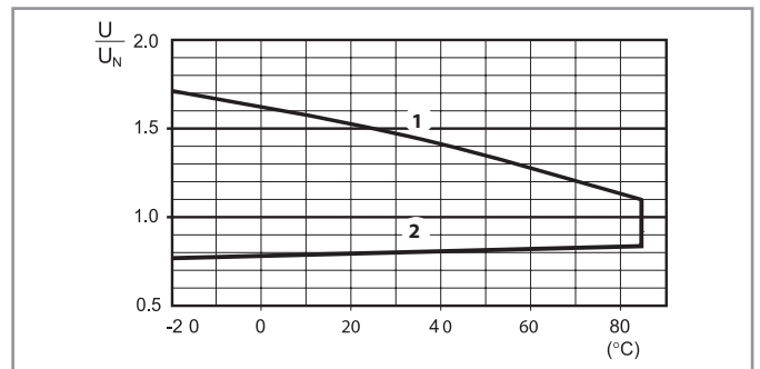
R 55 - AC coil operating range v ambient temperature
