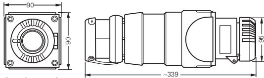
Coupler 4-pole
