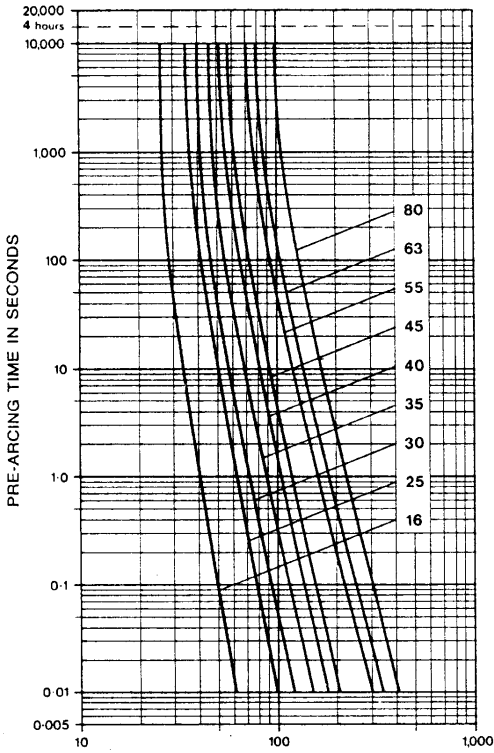
RMS SYMMETRICAL PROSPECTIVE CURRENT IN AMPERES
