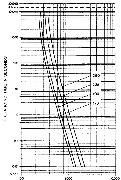
RMS SYMMETRICAL PROSPECTIVE CURRENT IN AMPERES
