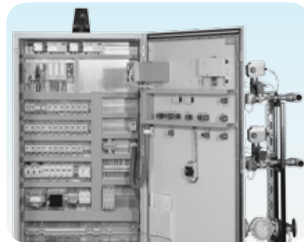
TC 4 installed in control cabinet by securing the lower section with screws or snapping it on to a DIN rail
