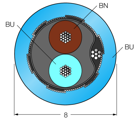
Cable Cross-section
