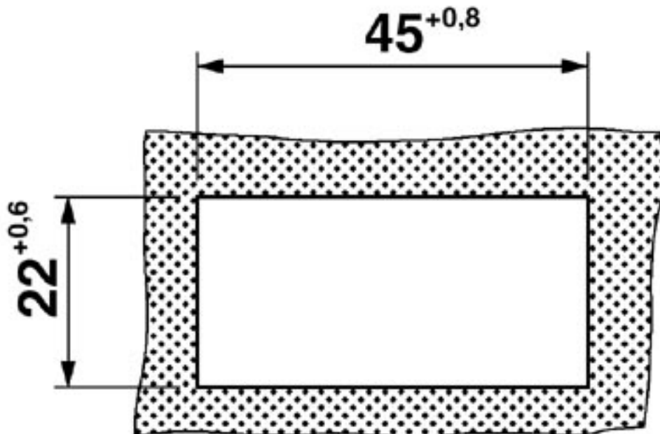
Dimensional drawing
