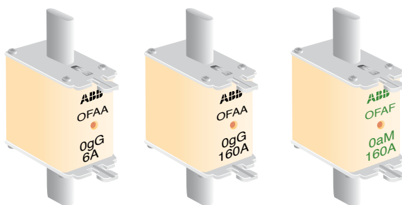
▲ The DIN 0 size fuse links for current range 6...250 A
