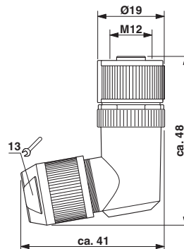
Socket M12-SPEEDCON, angled, shielded
