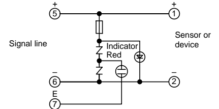
Control power supply 48V, 100V AC/DC
