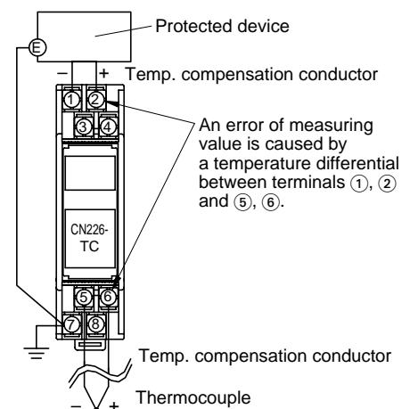
Note for thermocouple CN226-TC
