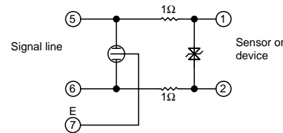
Signal line 24V, 48V DC
