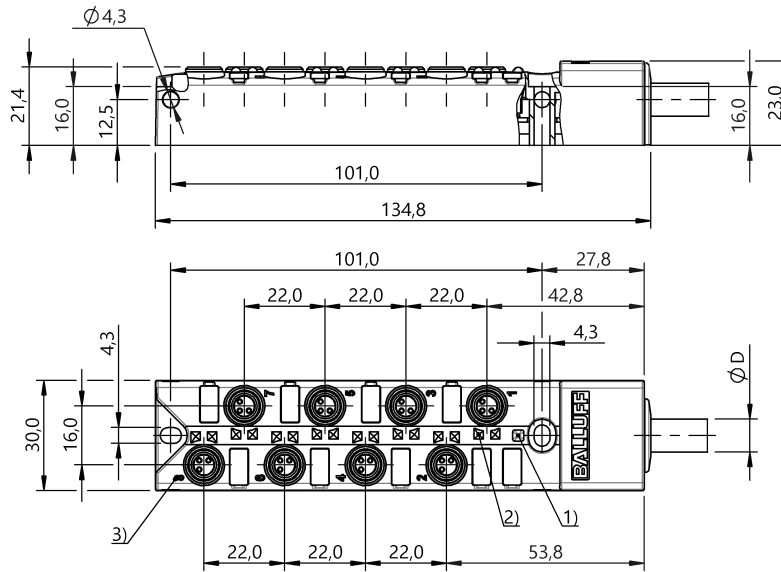
1) Power green 2) LED yellow for Signal 1 (NO) 3) Slot numbering
