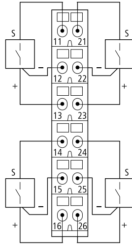
XN-S6...-SBBSBB for XN-4DI-24VDC-N
