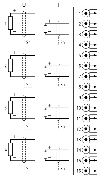
XNE-4AO-U/I
