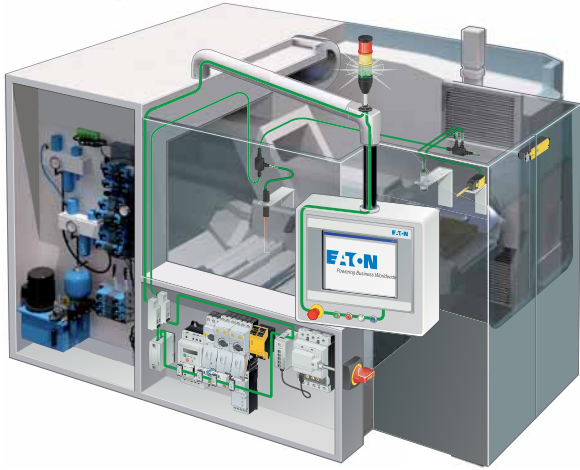
SmartWire-DT In-Panel and On-Machine Wiring Solution
