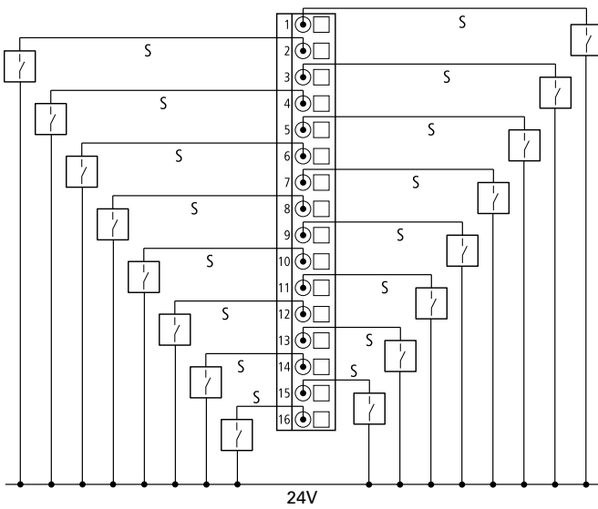
XNE-16DI-24VDC-P
