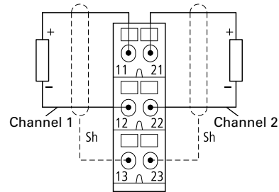
XNE-4AO-U/I
