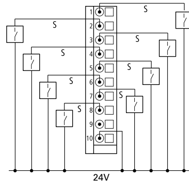
XNE-8DI-24VDC-P
