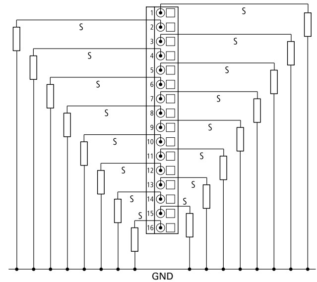
XNE-16DO-24VDC-0.5A-P
