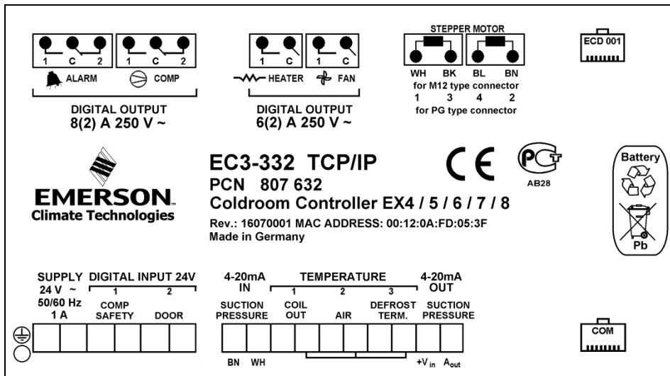
EC3-33x Coldroom Controller for Electrical Control Valves EX4 ... EX8
