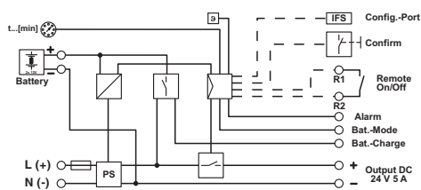
Block diagram
