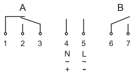
SC 44.21 pro (2 channels)
