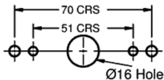
Panel Mounting With Oil Seal Drilling
