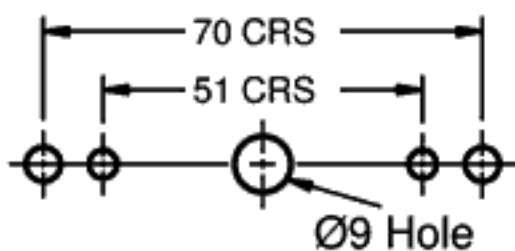
Std. Panel Mounting Drilling
