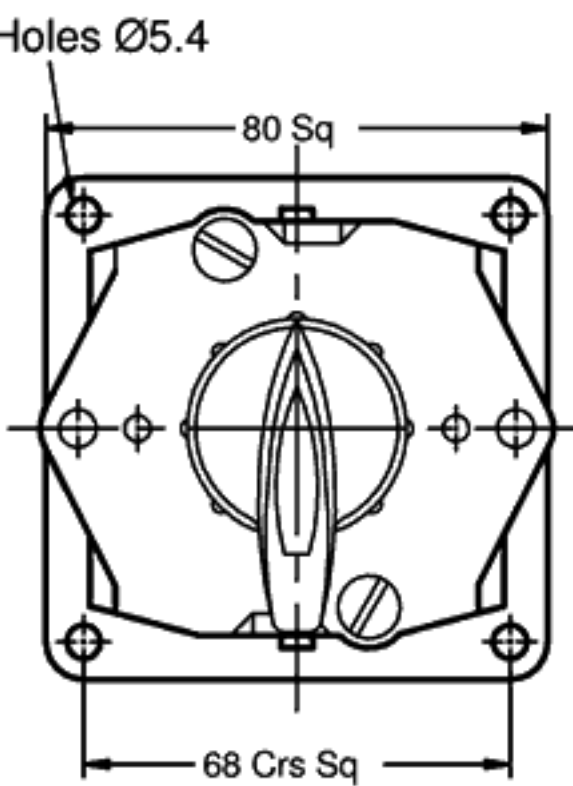
Panel Mounting With Oil Seal Drilling
