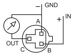
B (IN) C (OUT) A (GND)
