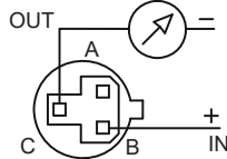
B (IN) C (OUT)
