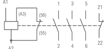
21-22 Normally Closed (NC) Auxiliary
