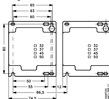
CI 32 – CI 50 with mechanical interlock Drilling dimensions
