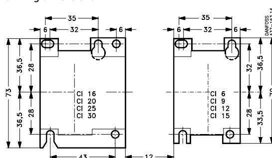
CI 6 – CI 30 with mechanical interlock Drilling dimensions
