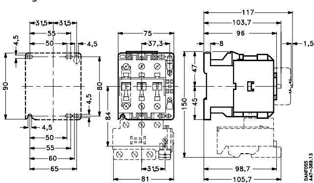
Contactors and motor starters CI 32, 37, 45, 50 Drilling dimensions
