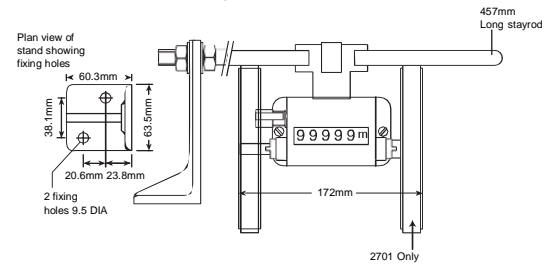
Product Dimensions 2401 | 2701
