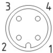
Contact arrangement
