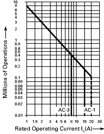
5.5kW contactors - AC1 & AC3 duty
