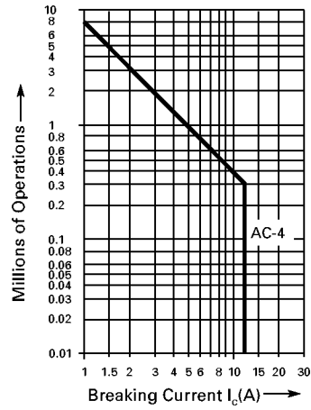
5.5kW contactors - AC4 duty
