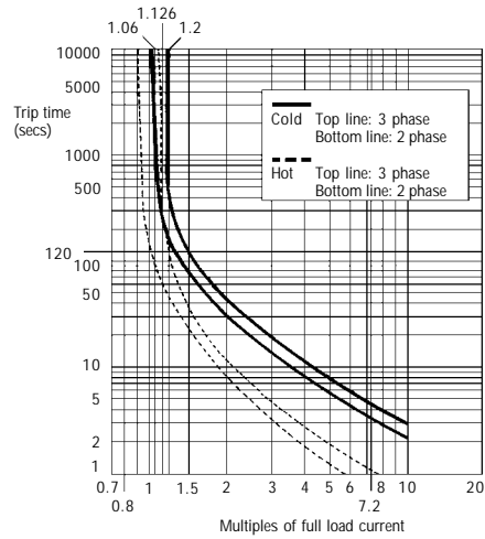
C316SNA3 thermal overload relay FLC current ranges 130 to 400A
