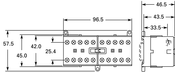
Mechanically Interlocked Contactors CE52BNC with Screw Pressure Plate and Quick Connect Terminals
