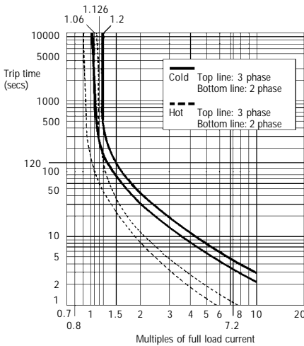
C316UNA3 thermal overload relay FLC current ranges 265 to 850A
