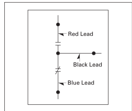
Figure 3-4. Switch Schematic
