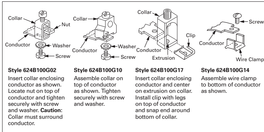
Figure 3-2. Terminals
