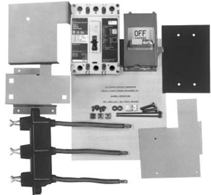
Type W Series C Retrofit Kit
