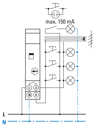
4-wire configuration
