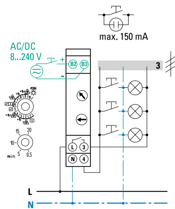
3-wire configuration
