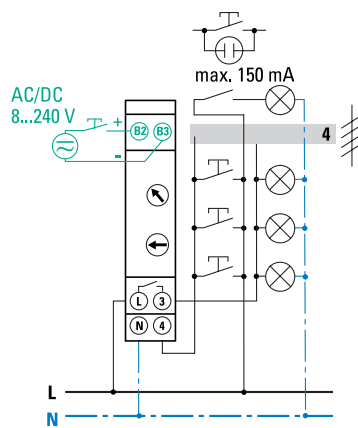
4-wire configuration
