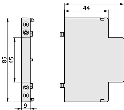
Auxiliary contact
