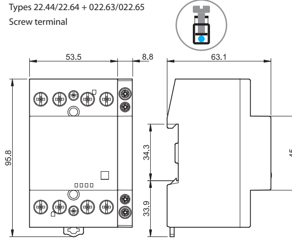
Types 022.63/022.65 Screw terminal
