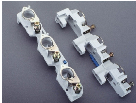
01492 CUSTO ® 60Classic D0-fuse base, busbar mounted, 27mm for busbar 10 mm E 18 / 3P
