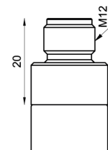
Connector M12-A, 4-pin, stainless steel (without LED)
