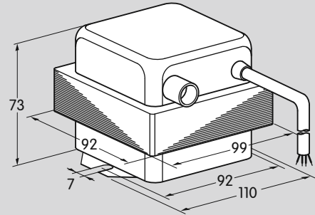
TZI 7,5-12/100, TZI 7,5-20/33
