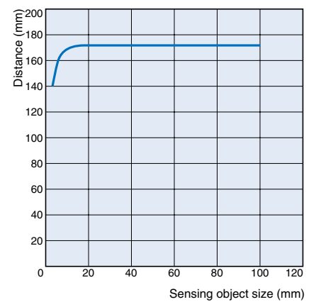
Narrow-beam E3Z-L
