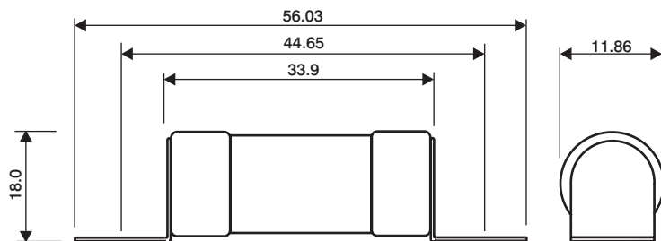
Offset Bolted Tag (OBT)
