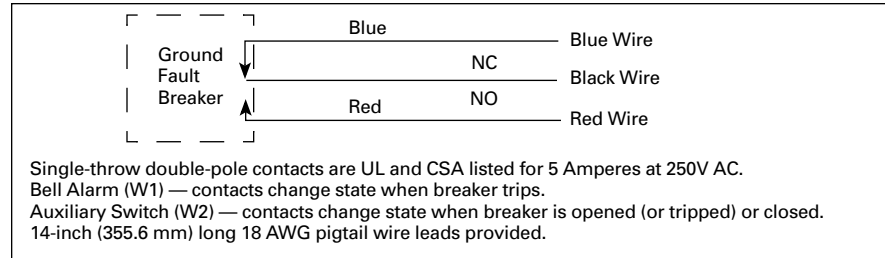
Figure 11-6. Bell Alarm and Auxiliary Contact Schematic
